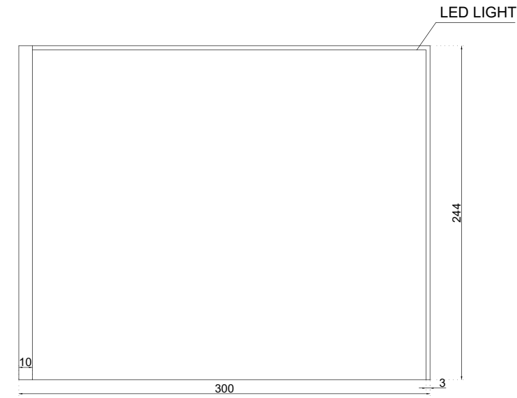
SIDE INTERFACE
