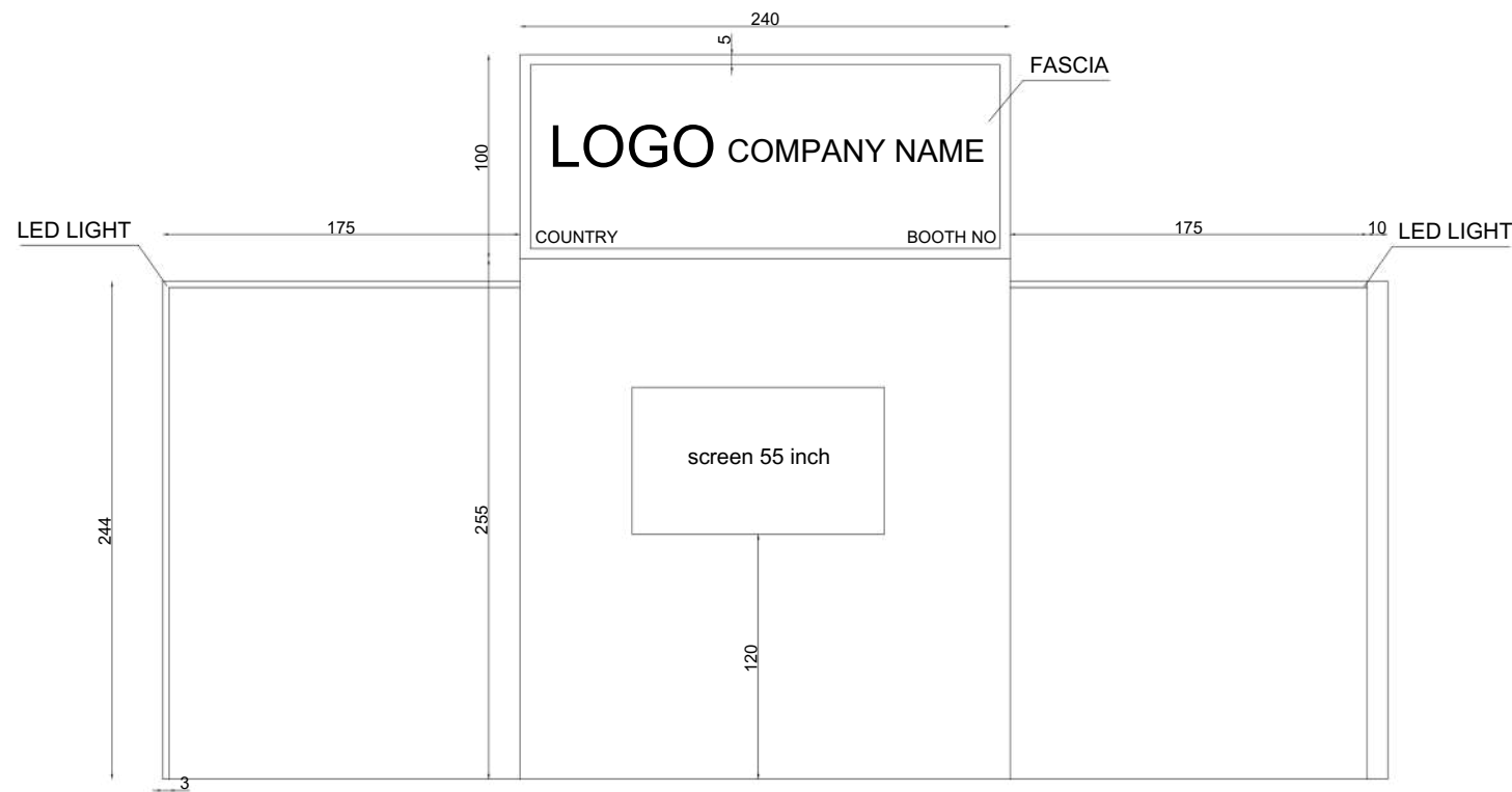
FRONT END
