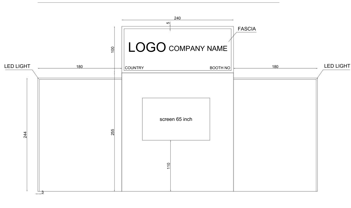
FRONT END
