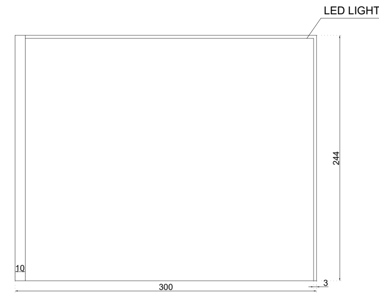
SIDE INTERFACE
