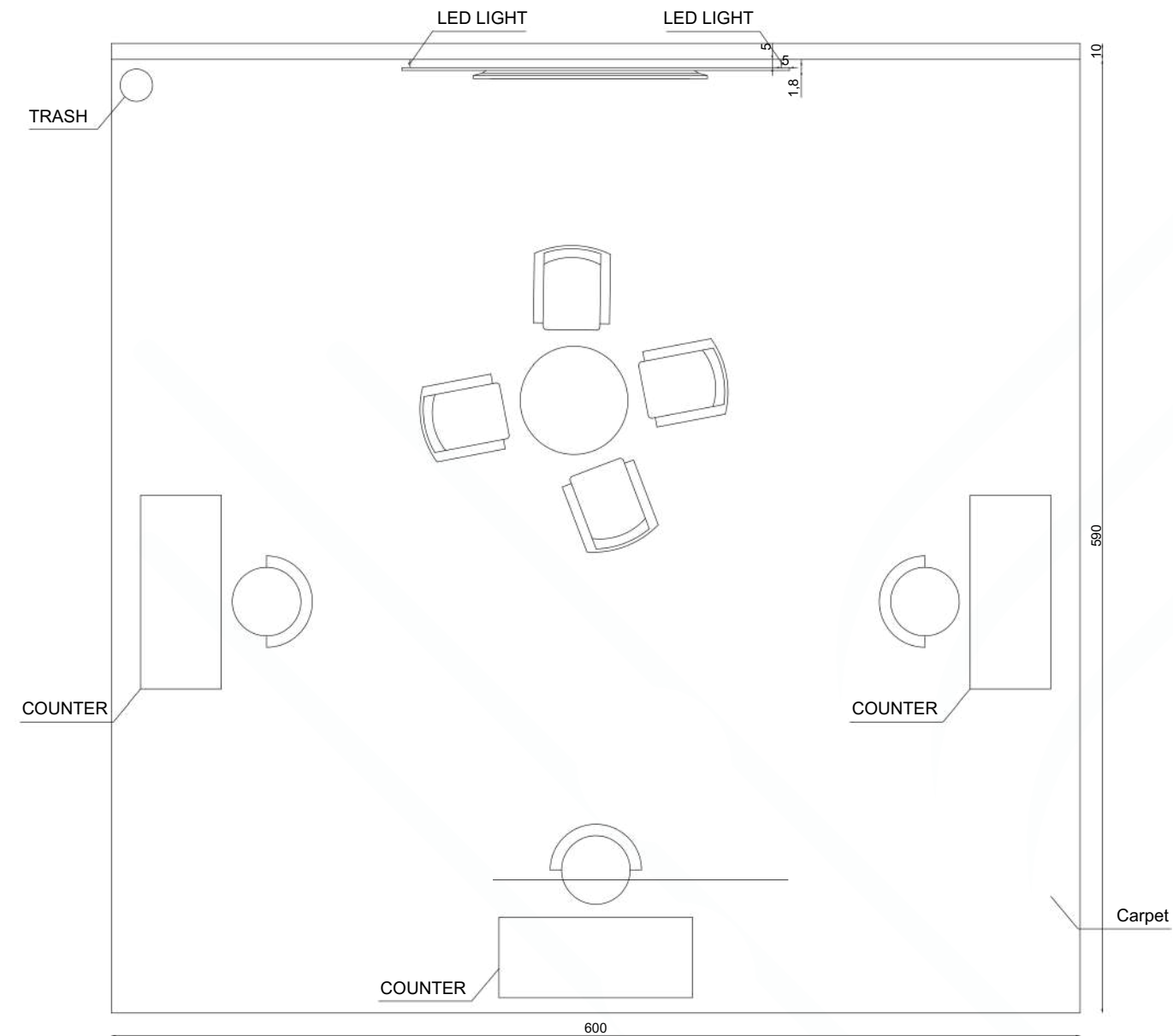
TOP VIEW
